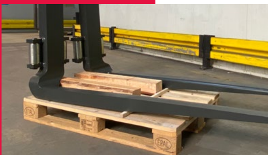
Cranked forks with inner radius relocated backwards
